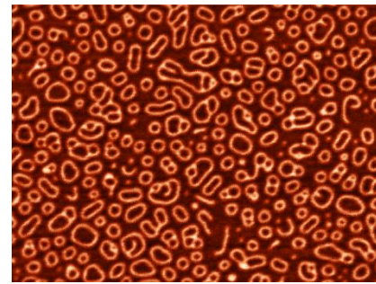
Ionic Assembly
