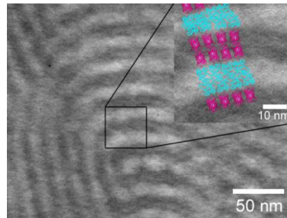
Enzyme Self-Assembly
