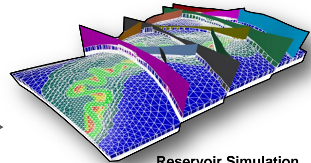
Reservoir Simulation
