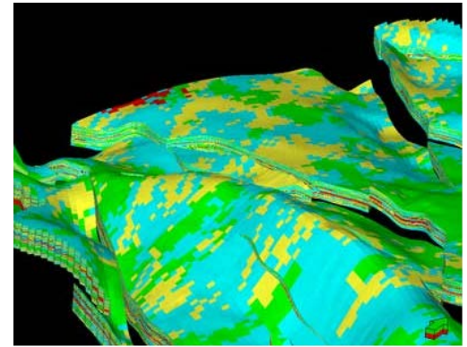
Geologic Modeling
