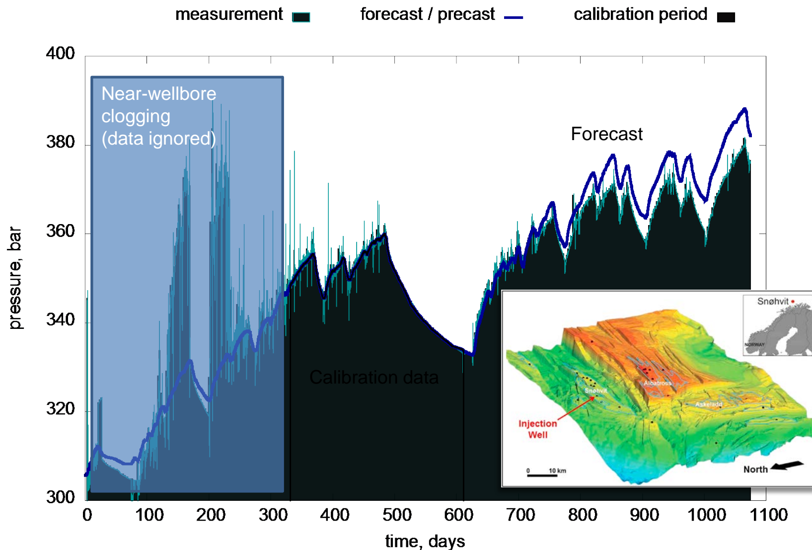
Figure: Reservoir pressure prediction using measured data at the Snøhvit CO 2 storage project. Model forecast is automatically updated as new injection data becomes available.
