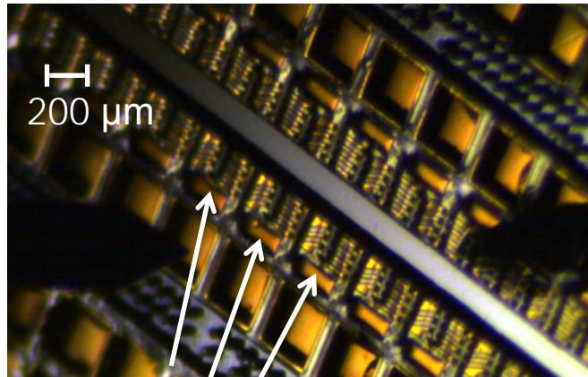
Batch-fabricated \mu electromagnets
