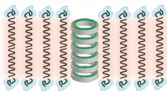
Artificial channels
