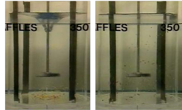
Baffles flat against the walls (unbaffled operation)
